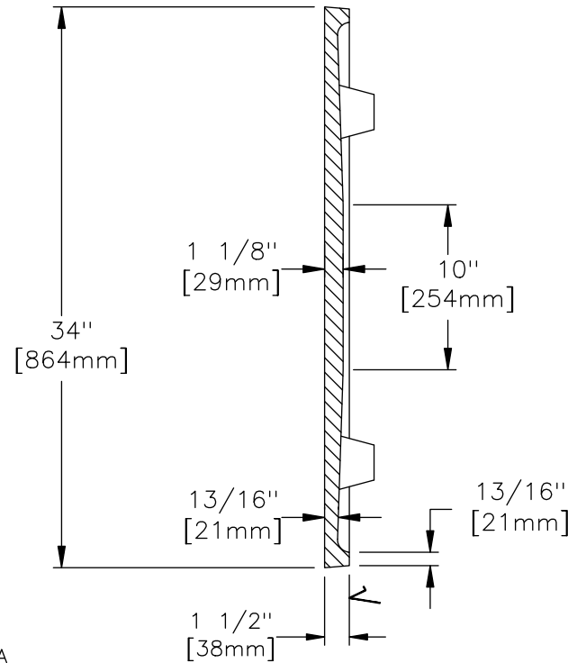
COVER SECTION
