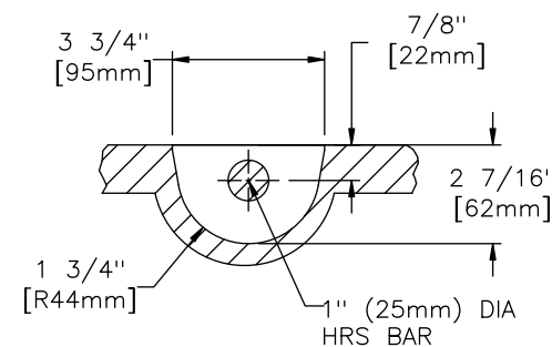
PICKBAR DETAIL
